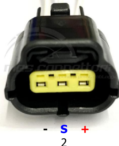
TE connectivity ECONOSEAL J codice: M174357-k CONTROPARTE: M174359-K
